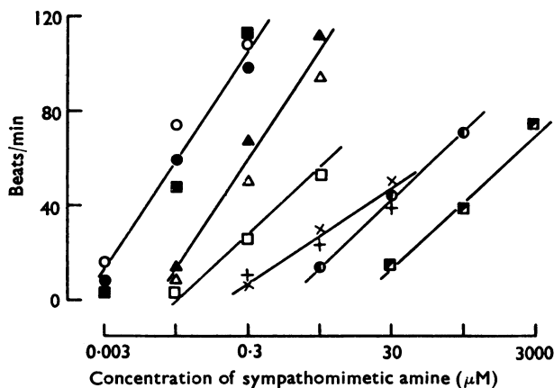
FIG. 2. Accelerator effect of 10 \mu M tyramine on isolated atria of reserpinized rats after previous exposure to various sympathomimetic amines. \bullet , Noradrenaline; \circ , noradrenaline + iproniazid (IPN); \odot , \alpha -methyl-noradrenaline; \blacksquare , adrenaline; \square , adrenaline + IPN; \blacksquare , dihydroxyphedrine; \triangle , dopamine + IPN; \blacktriangle , \alpha -methyldopamine; \times , norphenylephrine + IPN; + , metaraminol.
