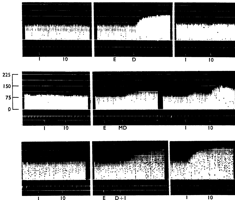
FIG. 1. Effect of dopamine and \alpha -methyldopamine on the tyramine chronotropic effect of isolated atria of rats pretreated with reserpine. Upper record in each row, beats/min (scale on left); middle record, time in min; lower record, signal. The left column tracing in each row indicates the control responses to 1 and 10 \mu M tyramine, and the right column the tyramine responses after exposure of the atria to 3 \mu M dopamine (D) in the middle panel of the first row, 0.3 \mu M \alpha -methyldopamine (MD) in the second row and 3 \mu M dopamine after 0.5 mM iproniazid (D+I) in the third row. E=3 \mu M disodium ethylenediamine tetraacetic acid.
